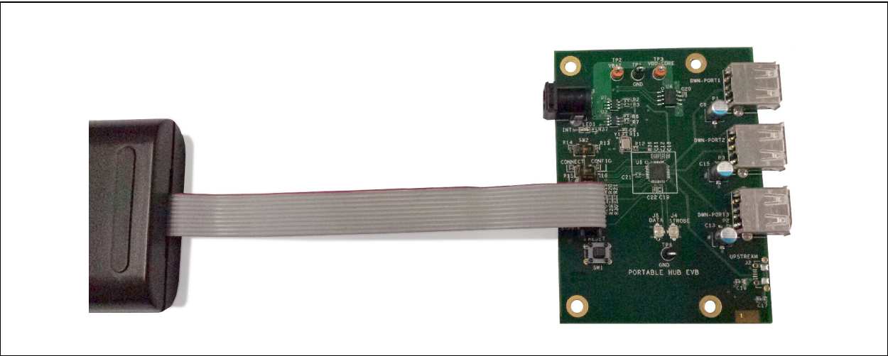
FIGURE 3-1: AARDVARK CONNECTION
